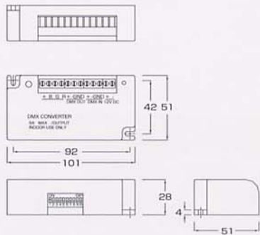
DMX Converter
