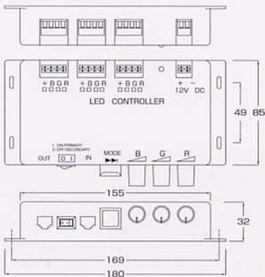
LED Controller
